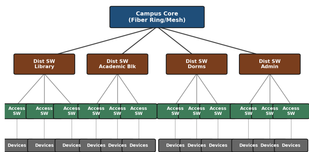
Hybrid Topology - University Campus (Core/Distribution/Access)
